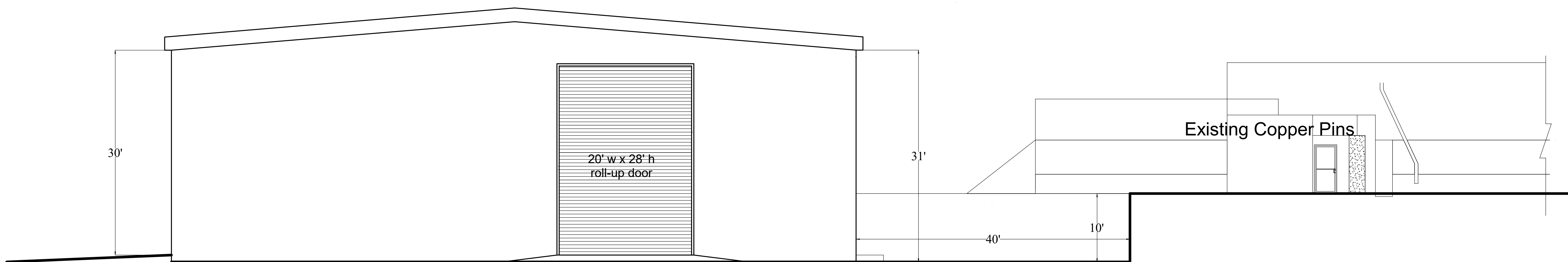
South Elevation
