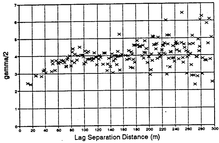
Angle Tol. = 10 degrees (anisotropic) N60E
