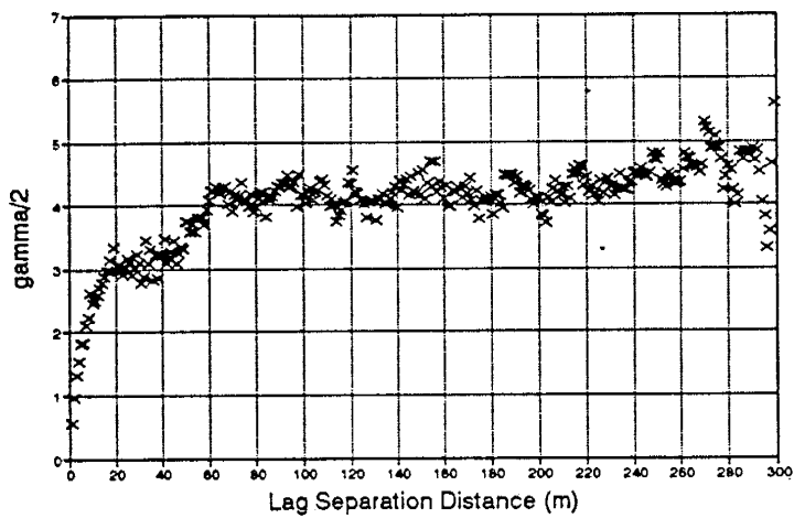
Vert. Distance Tol. = 1.0 m N60E
