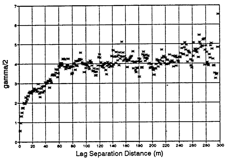
Direction N60E
