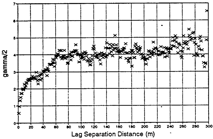
Vert. Distance Tol. = 0.25 m N60E
