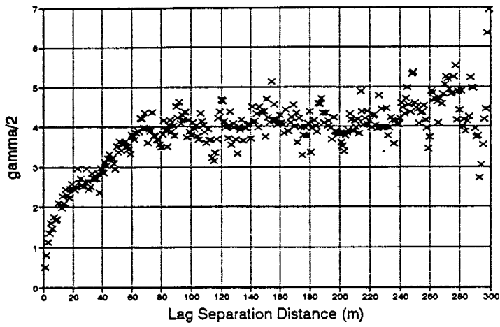
Vert. Distance Tol. = 0.10 m N60E
