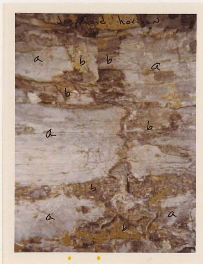
Figure 12. Arm-like extensions of jasperoid (b) in limestone (a).
