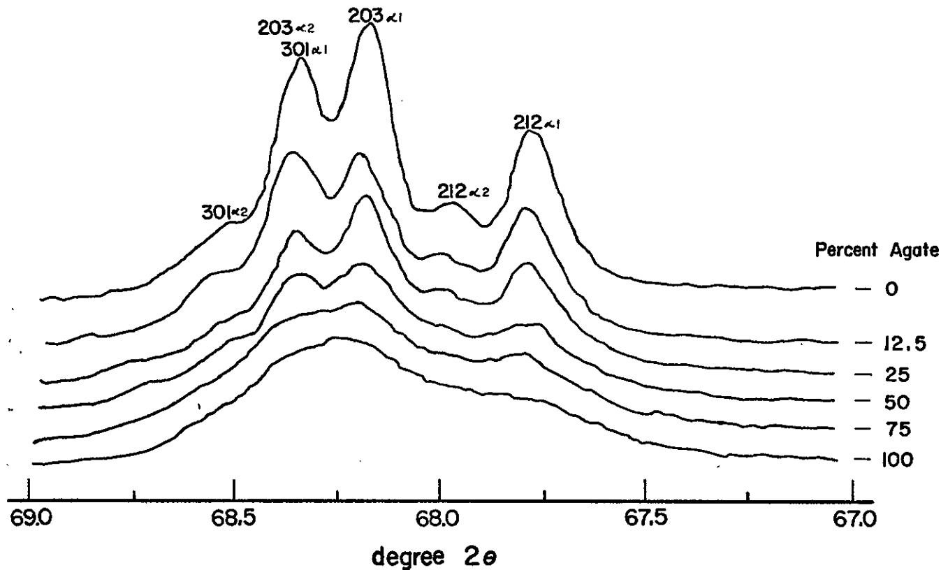
Figure 62. 68° quintuplet profiles for the six mixtures of quartz from the Ottawa Sandstone and Brazilian agate.
