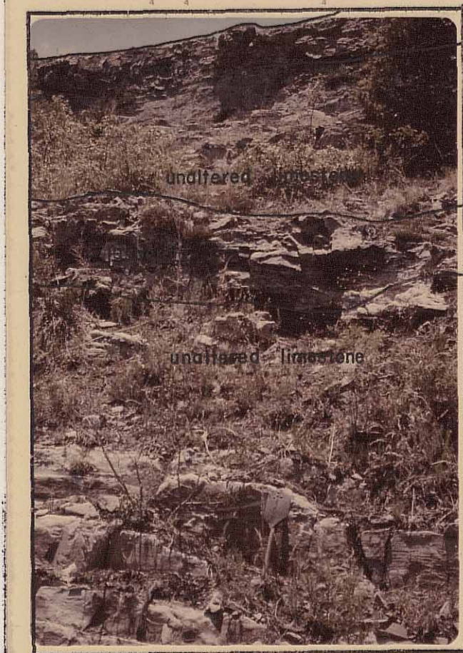
Figure 9a. Shows extensive silicification of the Kelly Limestone along the intersection of two faults which becomes localized in three horizons at some distance (approximately 30 feet) away from the faults. Outlined area represents Figure 9b.
