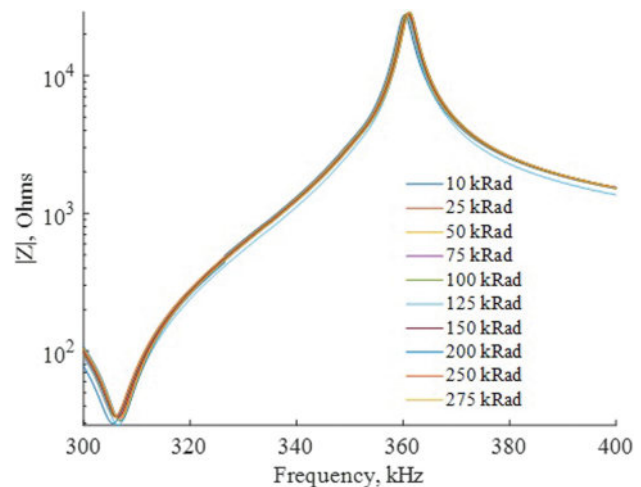
Fig. 8 Impedance magnitude data for sensor M2 at increasing absorbed gamma radiation dose
