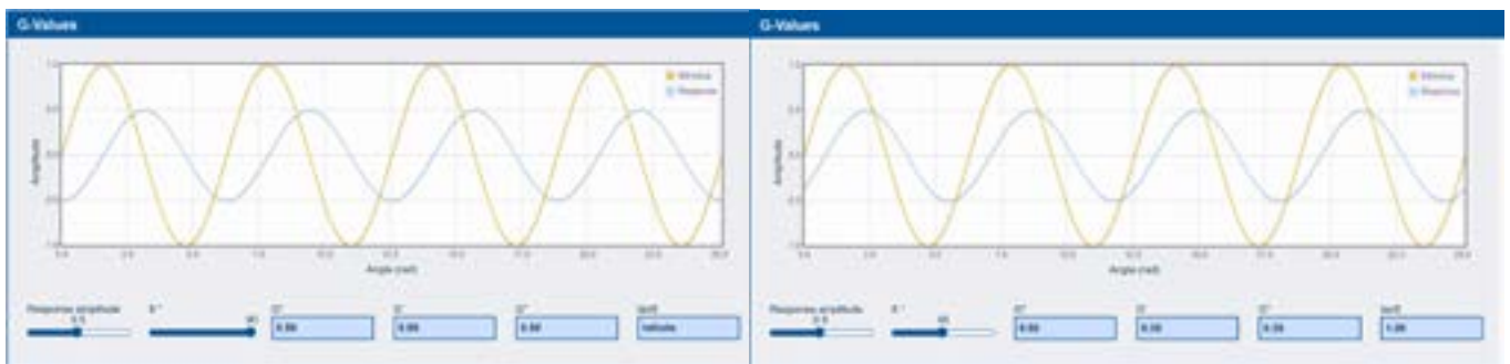
Figure 4-1 On the left we have the response 90^\circ out of phase - this is a pure viscous response. On the right the phase is 45^\circ and we have equal elastic and viscous components.
