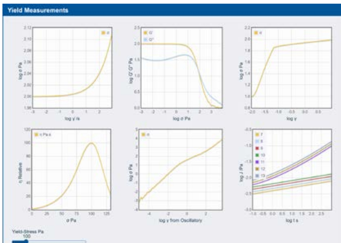
App 3-1 https://www.stevenabbott.co.uk/practical-rheology/Yield-Measurement.php
